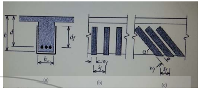
Figure 1: Illustration of the dimensional variables used in shear-strengthening calculations for repair, retrofit, or strengthening using FRP laminates.
