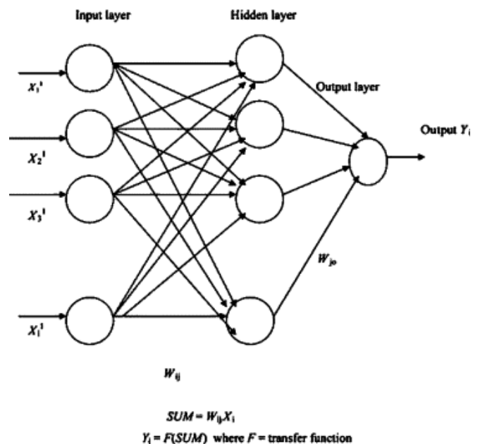
Figure 2: The basic architecture of multilayered ANN
