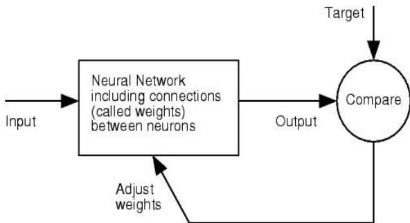
Figure 3: Back Propagation of multilayered ANN
