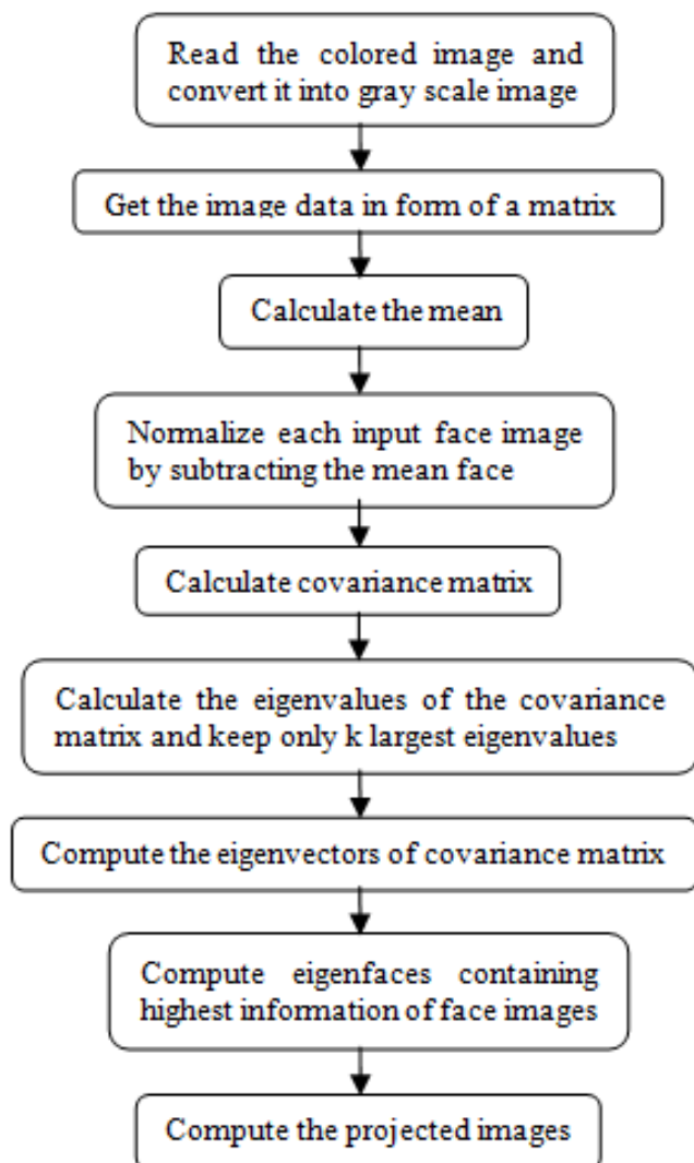
Figure 1: The basic architecture of PCA
