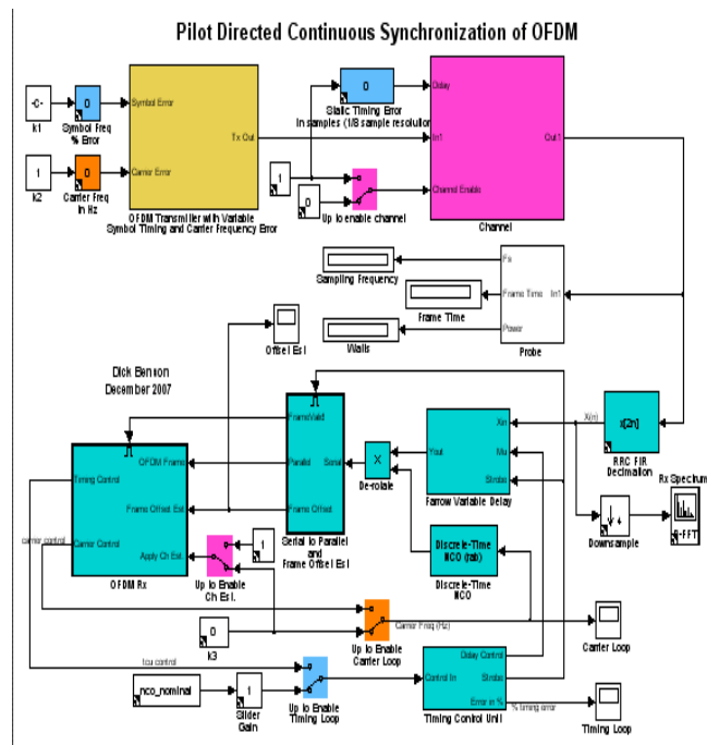
Figure 2: Pilot directed continuous synchronization of OFDM
