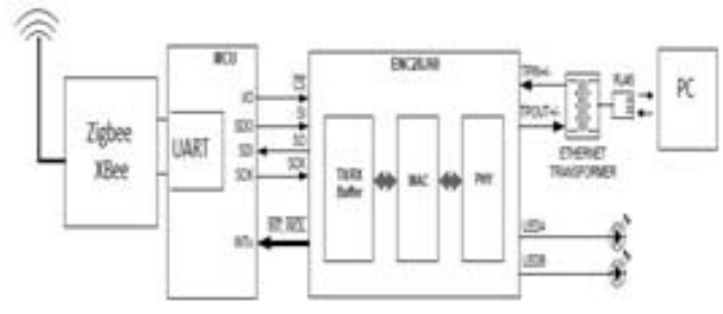
Figure 2: Ethernet web server Section
