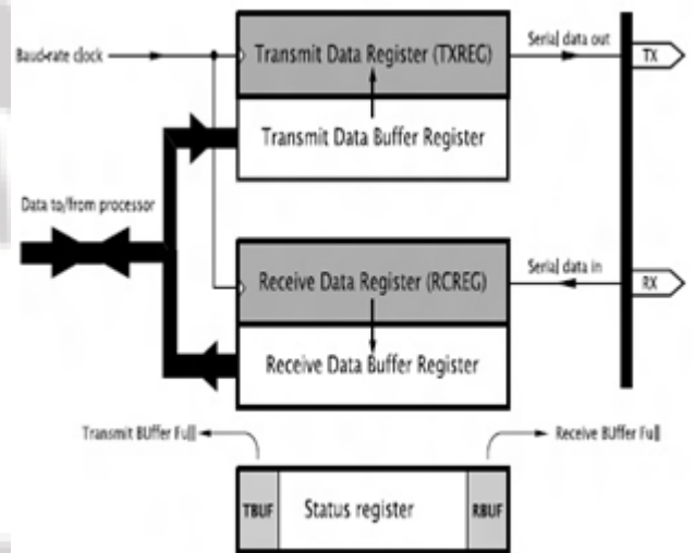
Figure 4: UART block diagram
