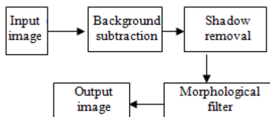
Figure 1: Silhouette extraction
