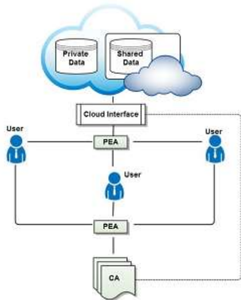
Figure 1: Secured Cloud Storage Framework (SCSF)
