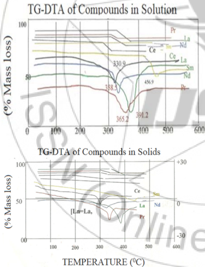
Fig.2. TG-DTA of Compounds of [Ln(SH)(OH)_2(H_2O)] Ln = La, Ce, Pr, Nd, Sm
