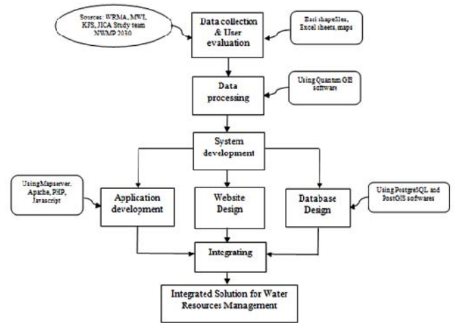
Figure 2: workflow diagram
