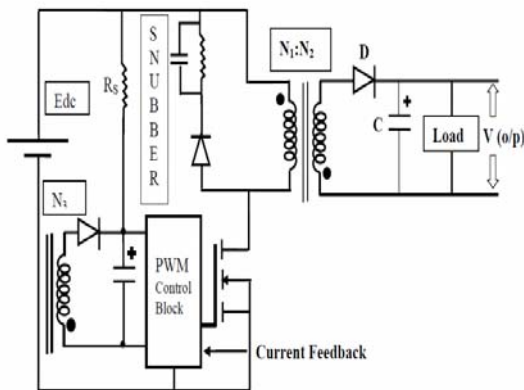
Figure 2: General circuit diagram of rectifier with PFC cells
