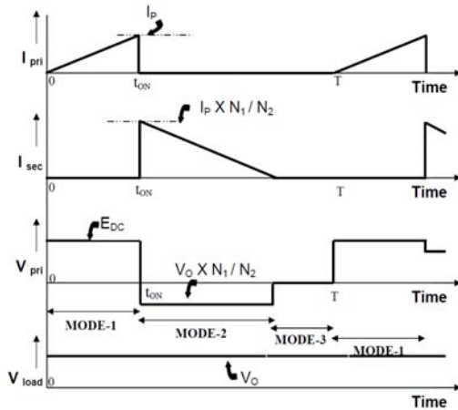
Figure 9: Fly-back circuit waveforms under discontinuous magnetic flux
