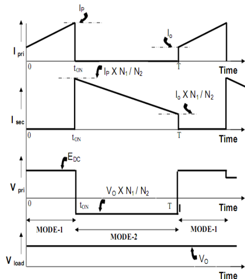
Figure 8: Wave forms for Fly-back circuit waveforms under continuous magnetic flux
