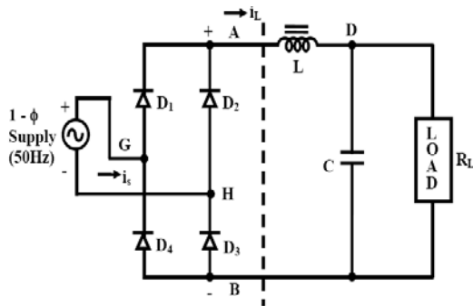
Figure 1: Full bridge diode rectifier
