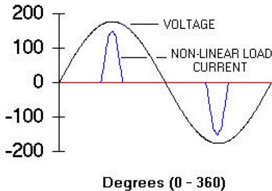
Figure 6: Voltage and current waveforms for non-linear loads
