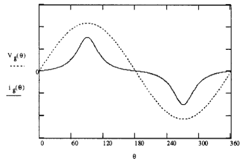
Figure 3: Typical input voltage waveforms for PFC.
