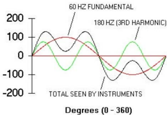
Figure 7: Waveform with symmetrical harmonic component
