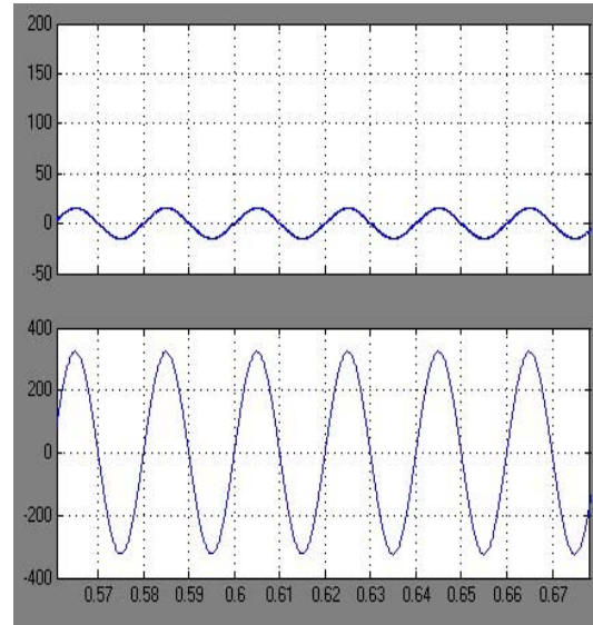
Figure 10: input current & input voltage measurement at diode rectifier
