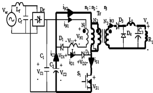
Figure 4: Family circuits have PFC function
