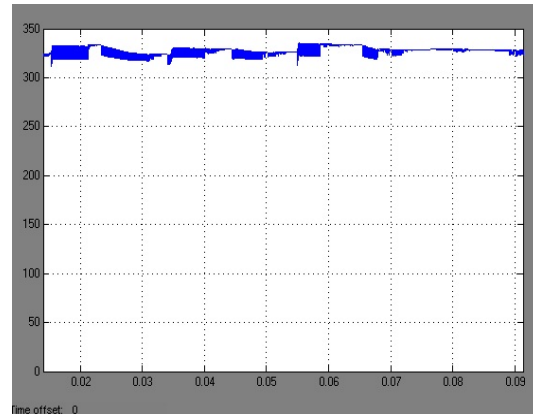
Figure 11: dc- capacitor voltage
