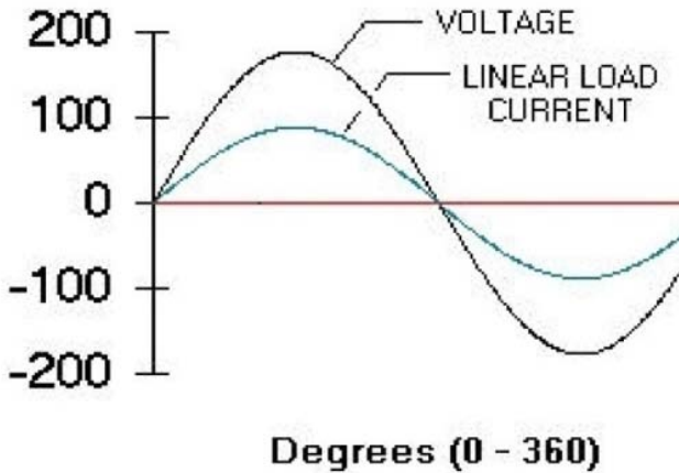
Figure 5: Voltage and current waveforms for linear loads
