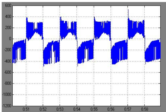
Figure 13: input current of inductor-transformer
