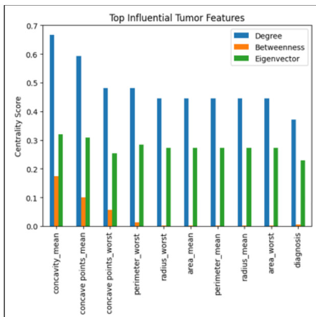
Figure 3: Centrality Analysis
