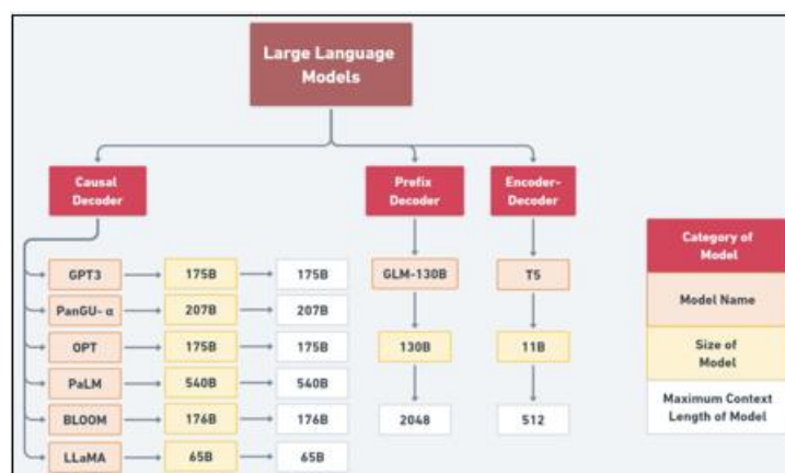
Figure 2.1: Representative Examples of Popular Large Language Models (LLMs)
