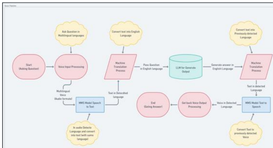
Figure 3.1: Basic pipeline for QA system using LLM
