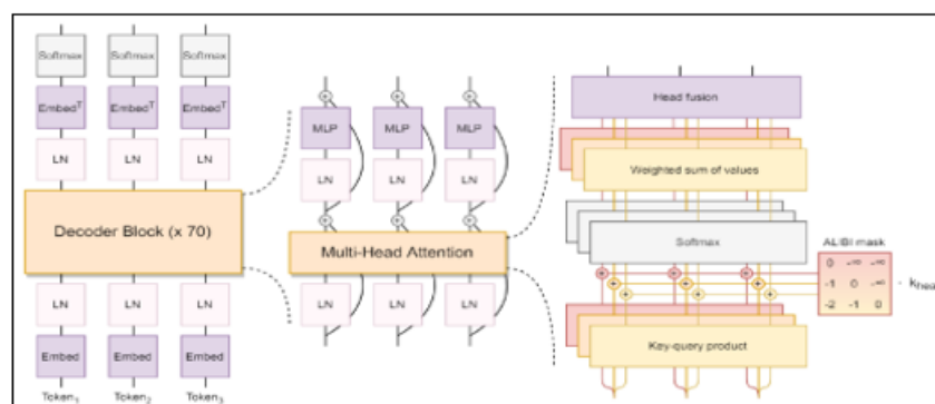
Figure 2.3: The BLOOM Architecture [22]
