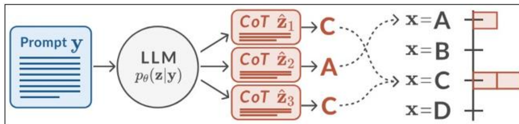
Figure 4.2: Generative process and answer likelihood (ensemble model, i.e., self-consistency).
