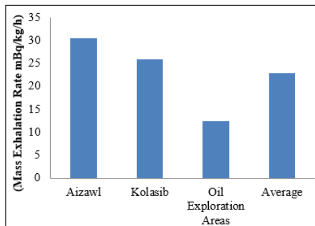
Figure 3: Comparison of the average values of radon mass exhalation rate in Aizawl District, Kolasib District and Oil exploration areas in Mizoram along with the overall average radon mass exhalation rate.
