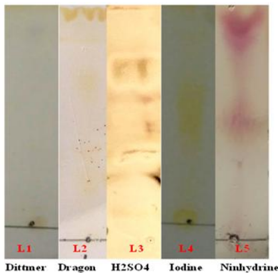
Figure I: TLC of lipids in Liver tissue stained with different reagents
