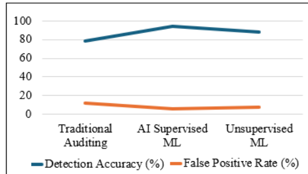
Figure 3: Accuracy Comparison
