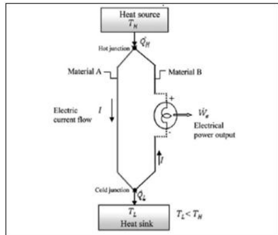
Figure 3: Working Principle
