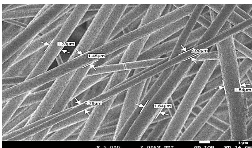
Figure 1(b): SEM image of (4:1wt%) PMMA/SrAl 2 O 4 :Eu 2+ , Dy 3+ fibre showing the diameter of fibre
