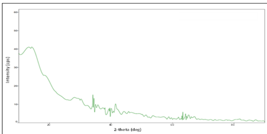
Figure 2: XRD graph image of (4:1wt%) PMMA/SrAl 2 O 4 :Eu 2+ , Dy 3+
