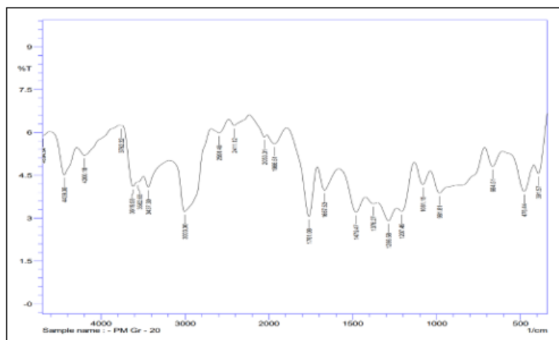
Figure 3: FTIR image of (4:1wt%) PMMA/SrAl 2 O 4 :Eu 2+ , Dy 3+
