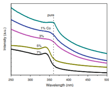
Figure 4: Co - doped ZnO nanoparticles' UV - vis spectra at ambient temperature
