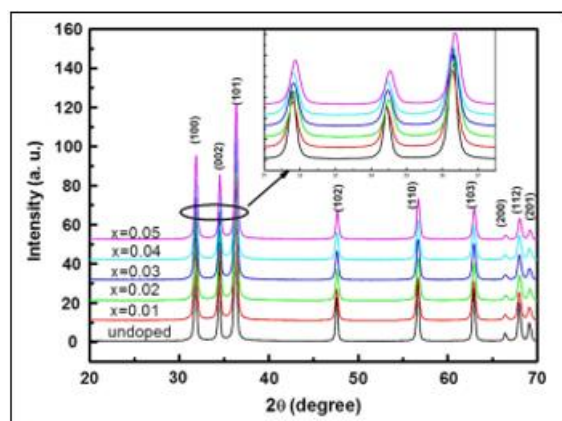
Figure 1: Zn 1-x Co x O nanoparticle XRD patterns
