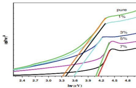
Figure 3: Variation in Co - doped ZnO nanoparticles' band gap
