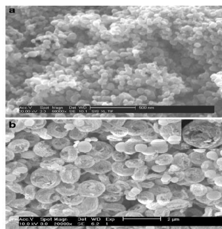
Figure 2: Co - doped ZnO nanoparticle SEM micrographs. a % and b % of Co
