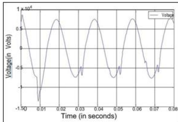
Figure 5: Voltage waveform with four wheelers connected
