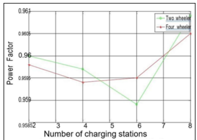
Figure 13: Power factor profile under peak load
