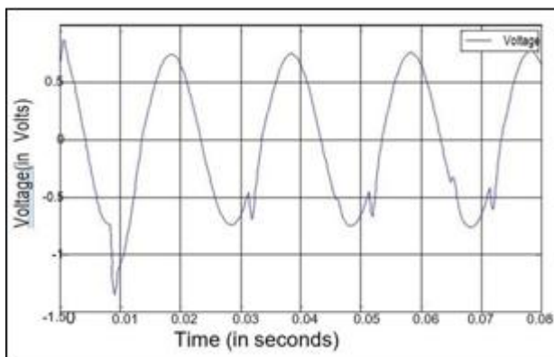
Figure 3: Voltage waveform with two wheelers connected
