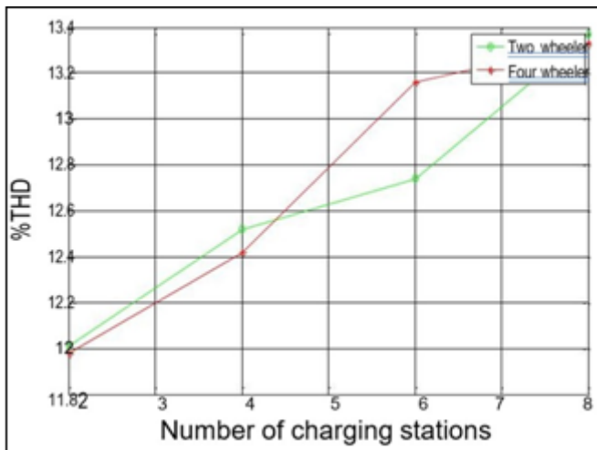
Figure 8: % THD profile under base load
