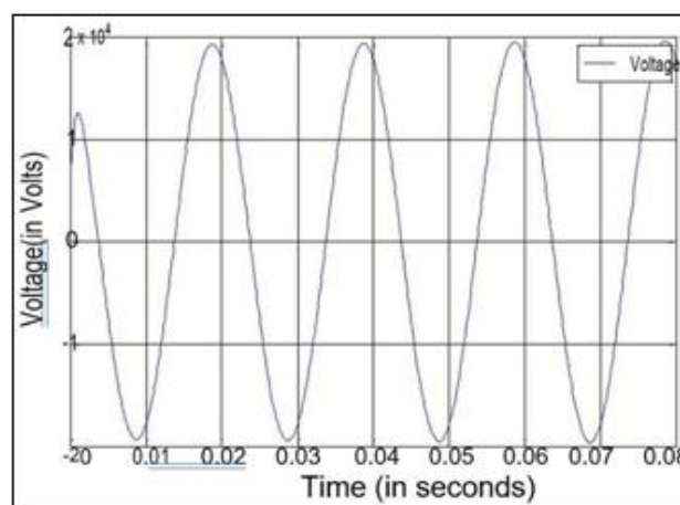
Figure 1: Voltage Profile
