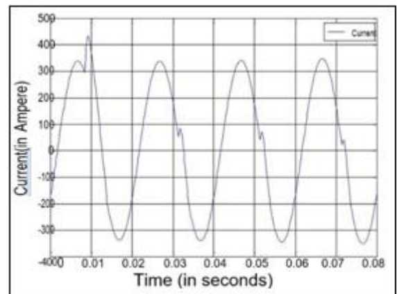
Figure 12: Current waveform with four wheelers connected
