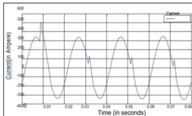
Figure 6: Current waveform with four wheelers connected
