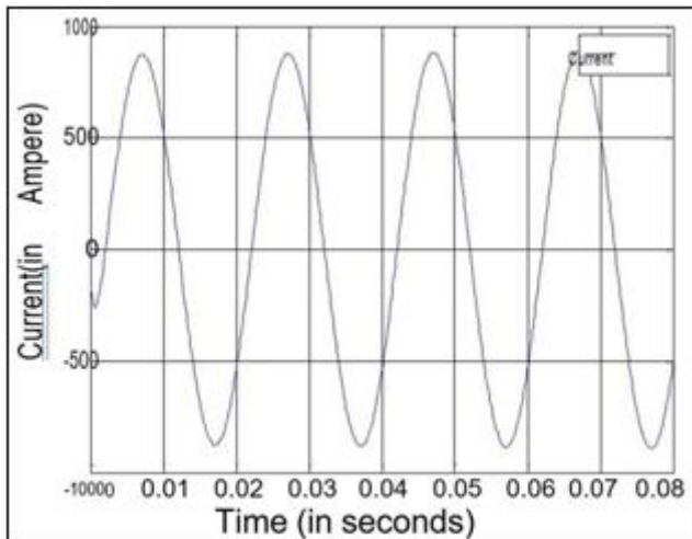
Figure 2: Current Profile
