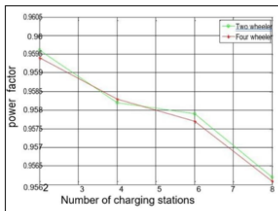
Figure 7: Power factor profile under base load
