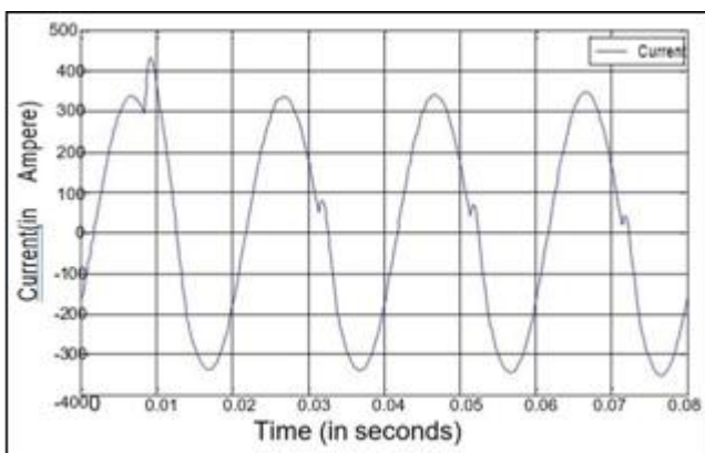
Figure 10: Current waveform with two wheelers connected
