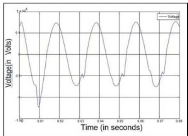
Figure 11: Voltage waveform with two wheelers connected
