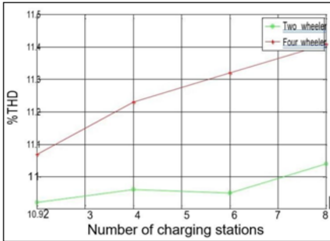
Figure 14: % THD profile under peak load
