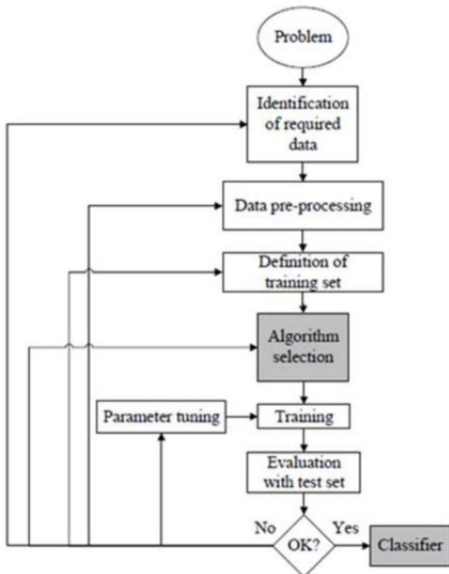
Figure 2: Workflow of supervised machine learning algorithm [4]
