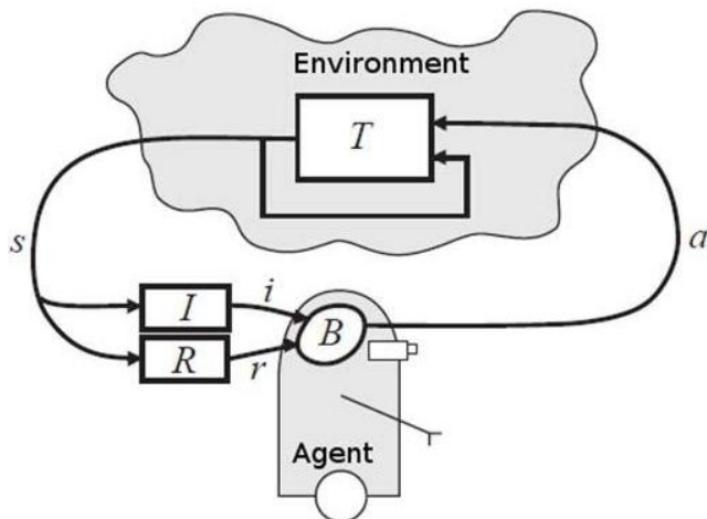
Figure 14: The Reinforcement Learning Model [18]
