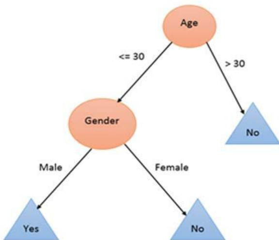
Figure 3: Decision Tree [5]
