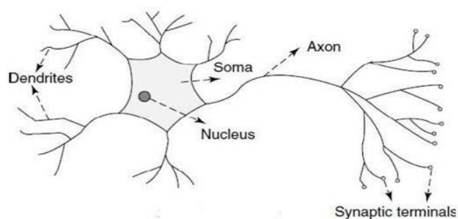
Figure 17: A Neuron [24]
