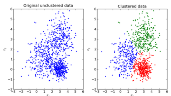
Figure 10: K-Means Clustering [12]
