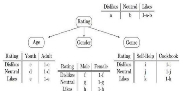
Figure 5: An Example of Bayesian Network [7]
