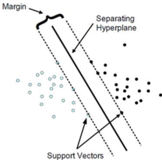
Figure 7: Working of Support Vector Machine [8]
