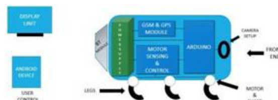
Figure 1: Block Diagram of proposed Robot
