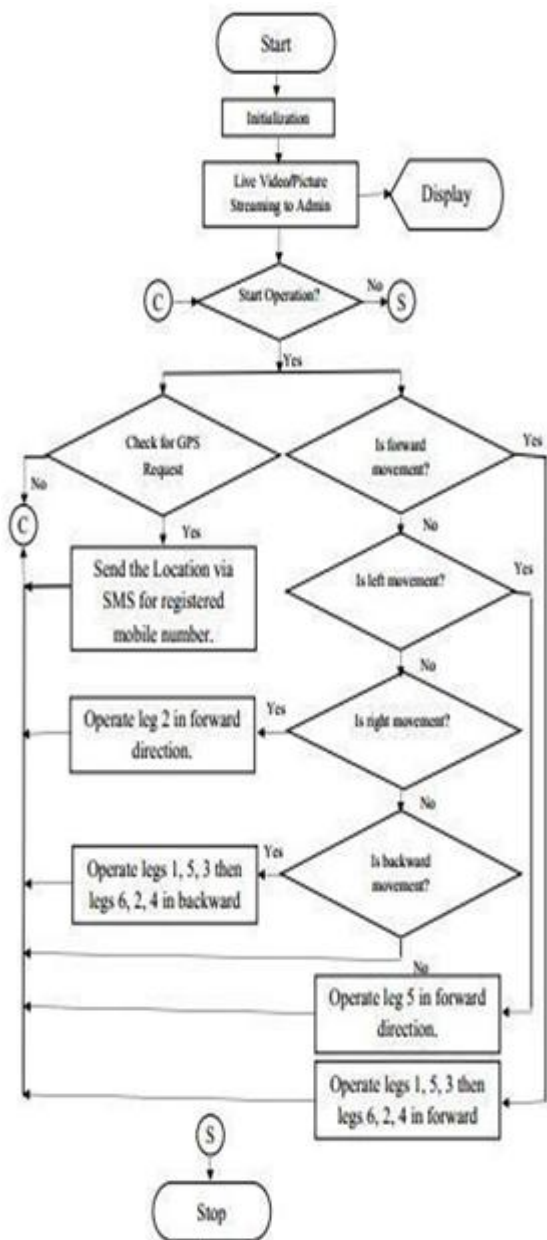
Figure 2: Represents the entire operation of the proposed robot, in a pictorial form. The circuit diagram for the work is shown in Fig. 3 and Fig. 4.
