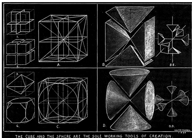
Figure 4: Cube-Sphere
