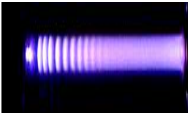
Figure 9: Gas discharge: light rings with own centers of gravity spinning in parallel planes which are normal to the gravity shaft, i.e., cathode-anode axis
