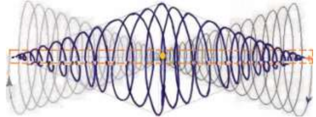
Figure 8: Electric bar with positive and negative electric vortices
