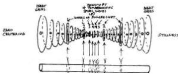
Figure 16: Gravity Bar
