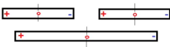
Figure 1: When opposite poles of two bar magnets are near enough to each other, they quickly move to each other and
