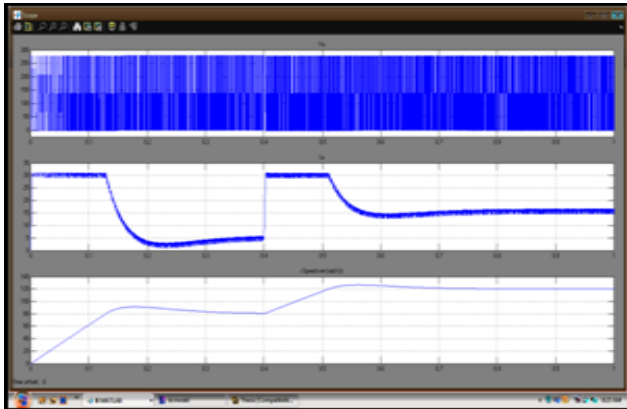
Figure 10: Simulink response of PID controller for T_L=5 to 17 Nm and speed (80 & 120 rad/sec)
