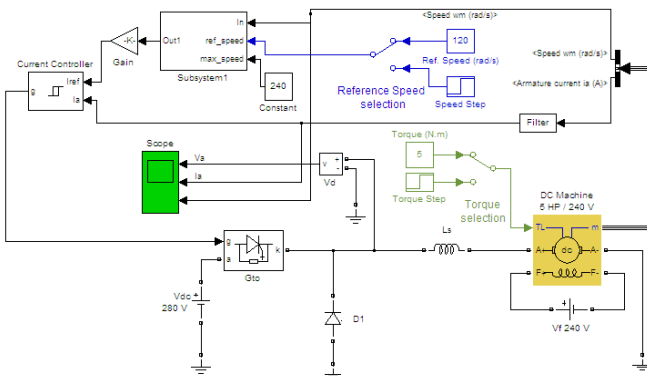
Figure 5: Matlab/Simulink model of SEDCM for Fuzzy logic controller
