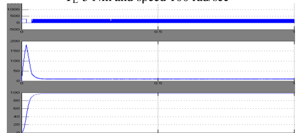
Figure 9: Simulink response of Fuzzy controller for torque T_L = 5 Nm and speed of 100 rad/sec
