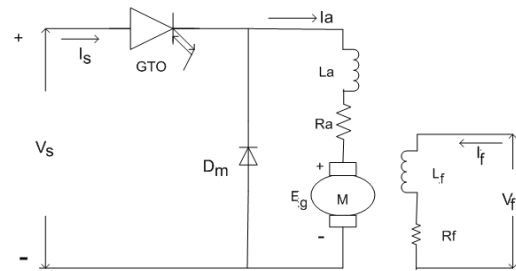
Figure 2: Chopper fed SEDC motor
