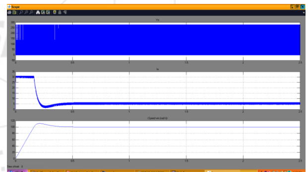
Figure 8: Simulink response of PID controller for torque T_L = 5 Nm and speed 100 rad/sec
