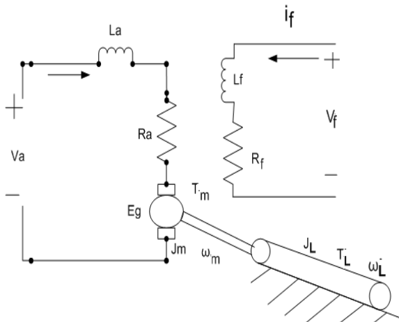
Figure 1: Dynamic model of separately excited DC
