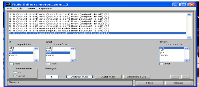
Figure 6: Fuzzy rules for 3 membership function
