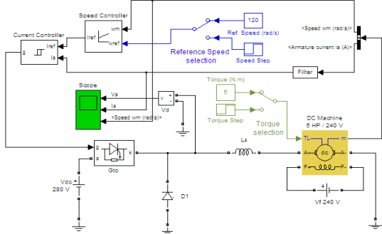
Figure 4: Matlab/Simulink model of SEDCM for PID controller
