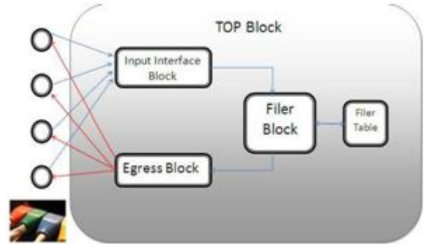
Figure 2: Interface diagram
