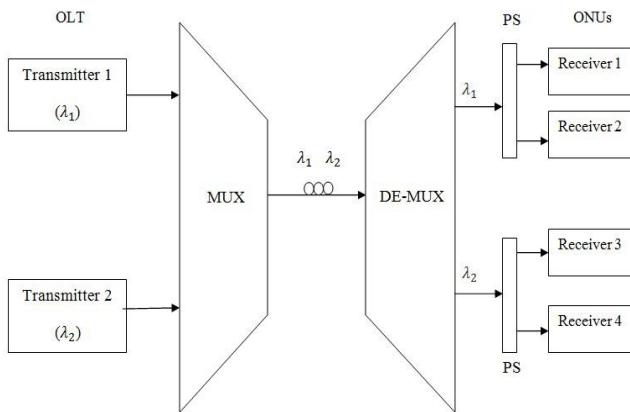
Figure 3: Block diagram of Hybrid WDM/TDM PON
