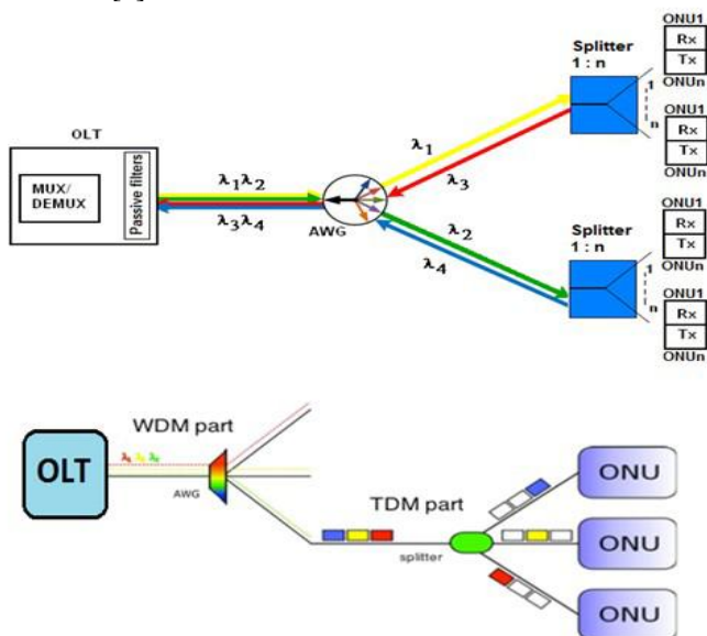
Figure 1: Hybrid WDM/TDM PON
