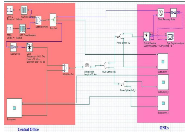
Figure 6: Simulation using Manchester coding
