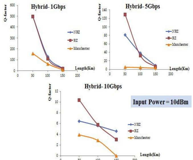
Figure 10: Comparison for different Bit Rates
