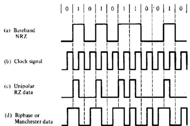
Figure 2: Different Coding Techniques
