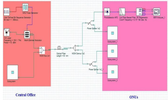
Figure 4: Simulation using NRZ coding
