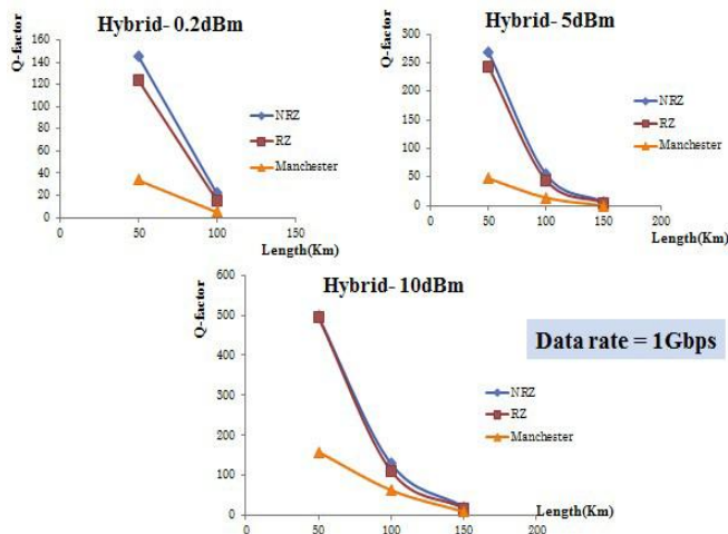
Figure 9: Comparison for different Power levels
