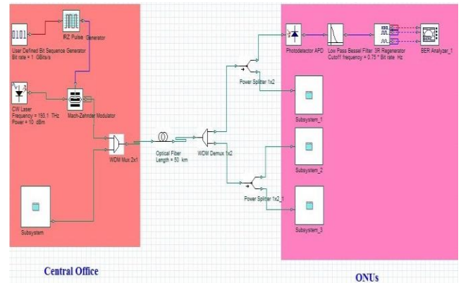
Figure 5: Simulation using RZ coding
