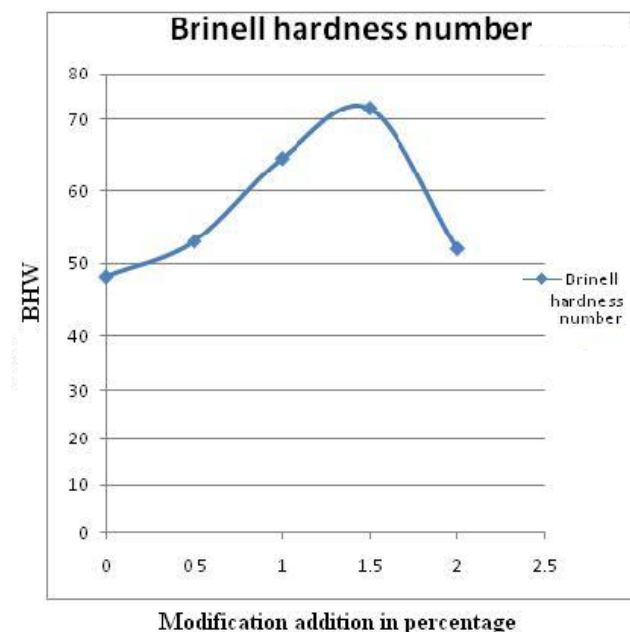
Figure 3: Relation between modifier addition and BHN
